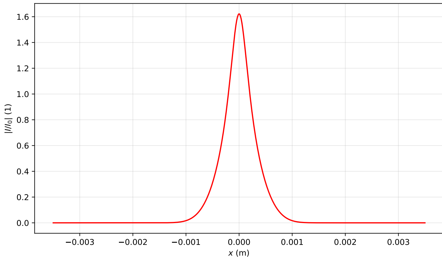
Intensity profile I(x, y = 0, z = 0.239)/I_0 , P_{in}=6.5P_{cr} , artificial time
